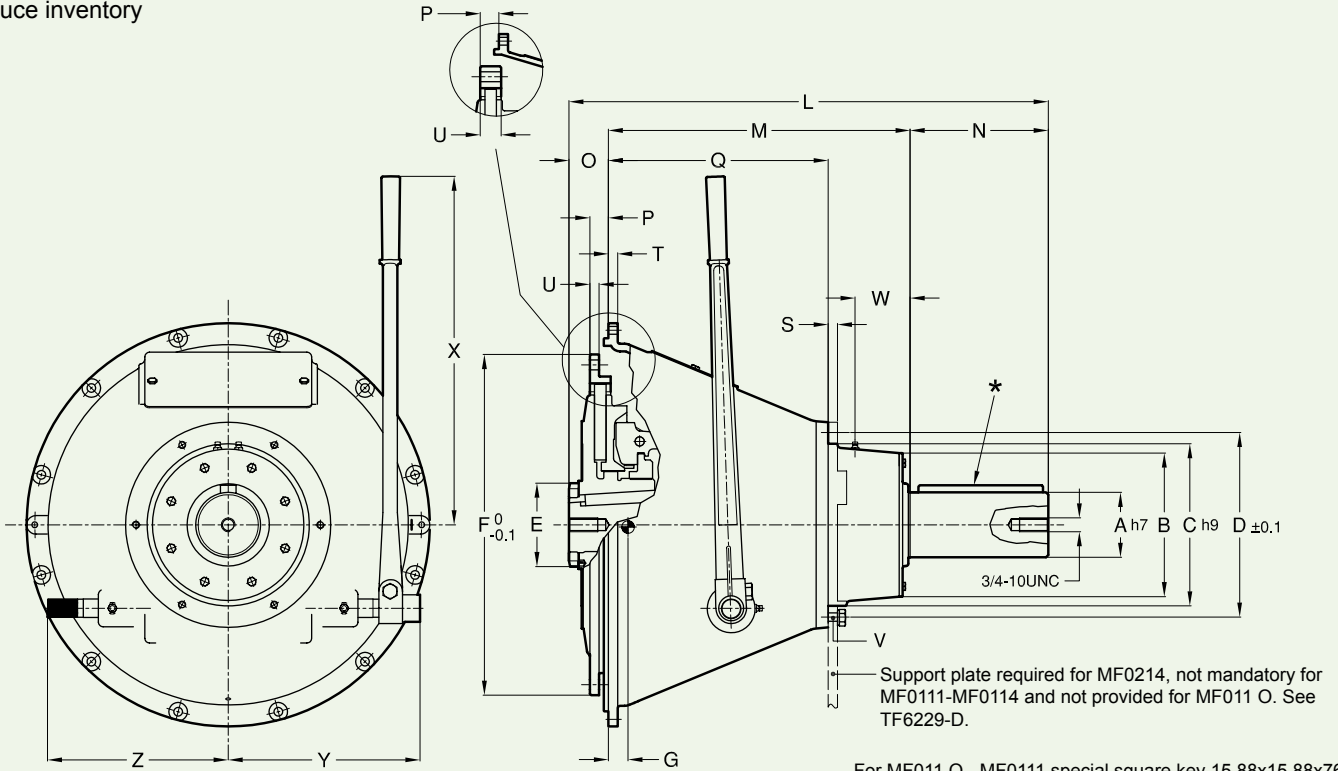
Dimensions (mm)
